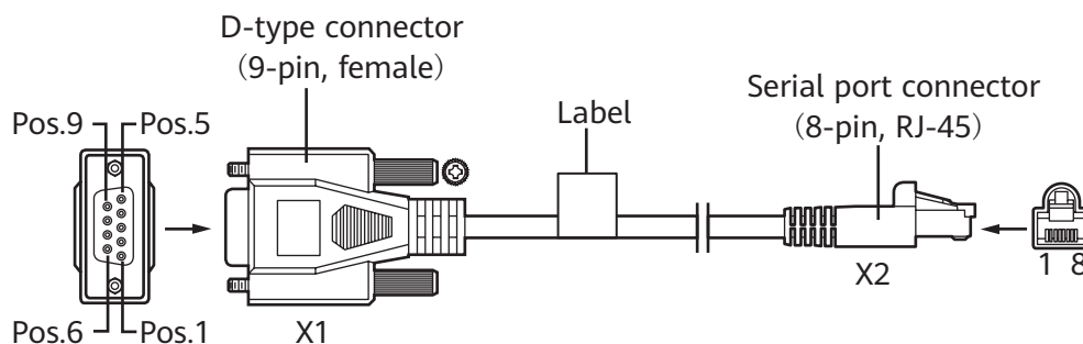
Figure 8-9 Structure of a console cable
