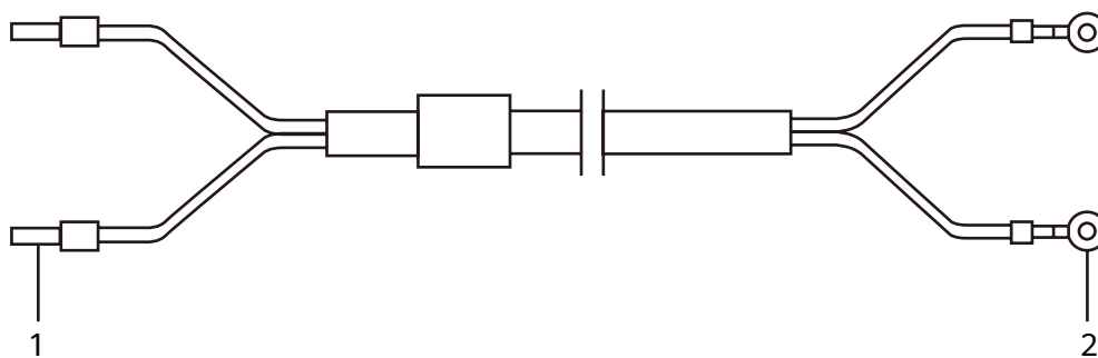
Figure 8-1 DC power cable with an OT terminal
