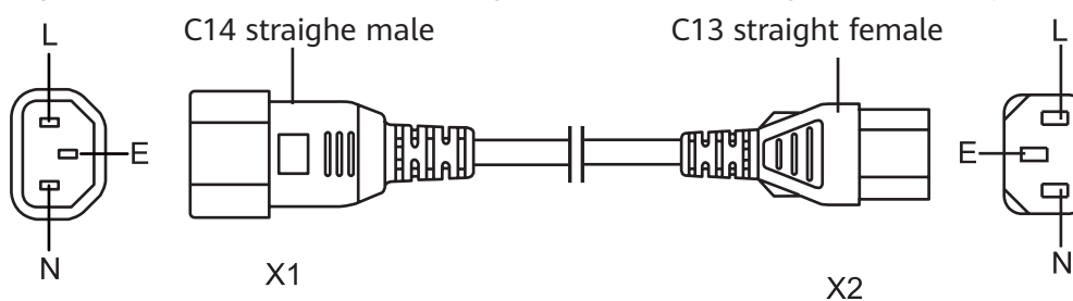
Figure 8-2 Structure of a C14 straight male to C13 straight female AC power cable
