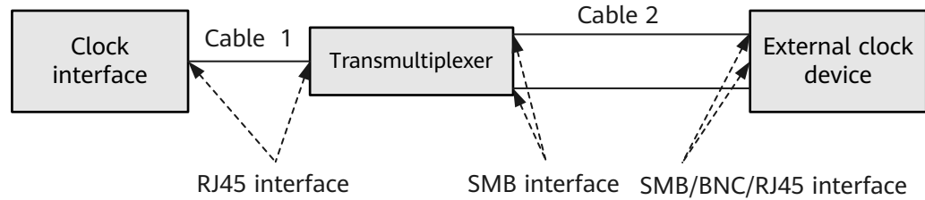
Figure 8-14 Clock cable connections
